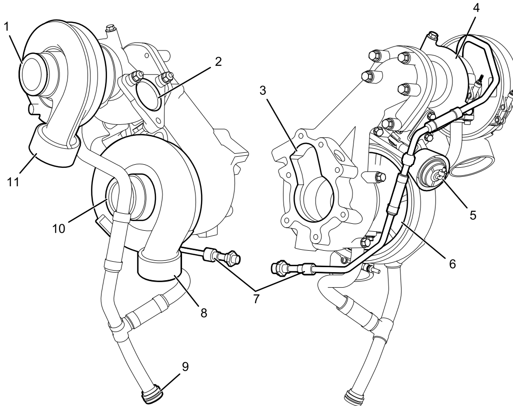
Figure 4 High and Low Pressure Turbocharger Components – Inner and Outer views
